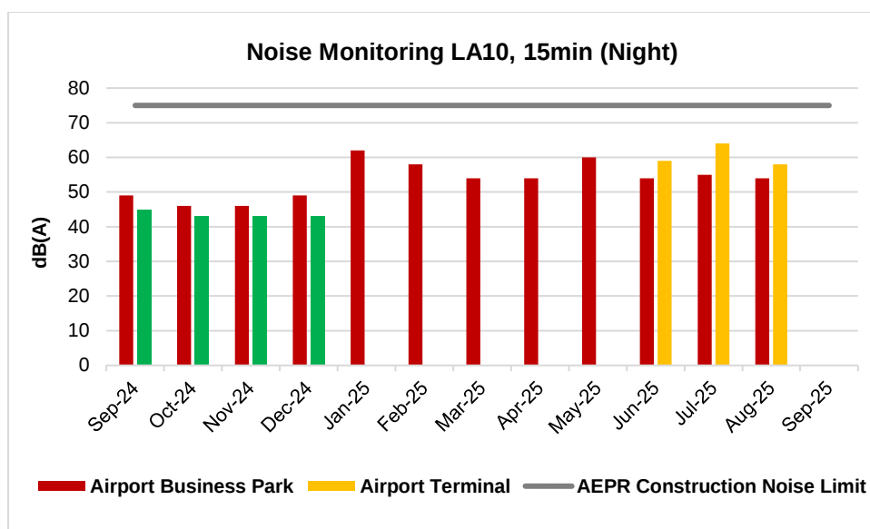
Figure 18: LA10 Noise Monitoring Results (Night)
