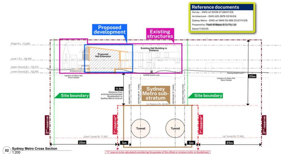
Figure E3 Cross-section showing Development envelope and relationship to Metro Infrastructure
