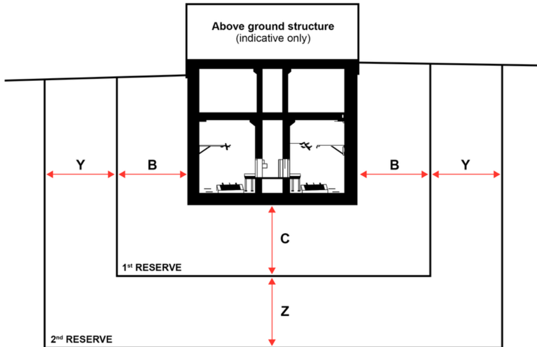
Figure 3.3 Protection reserves for metro shafts, dives and station boxes
