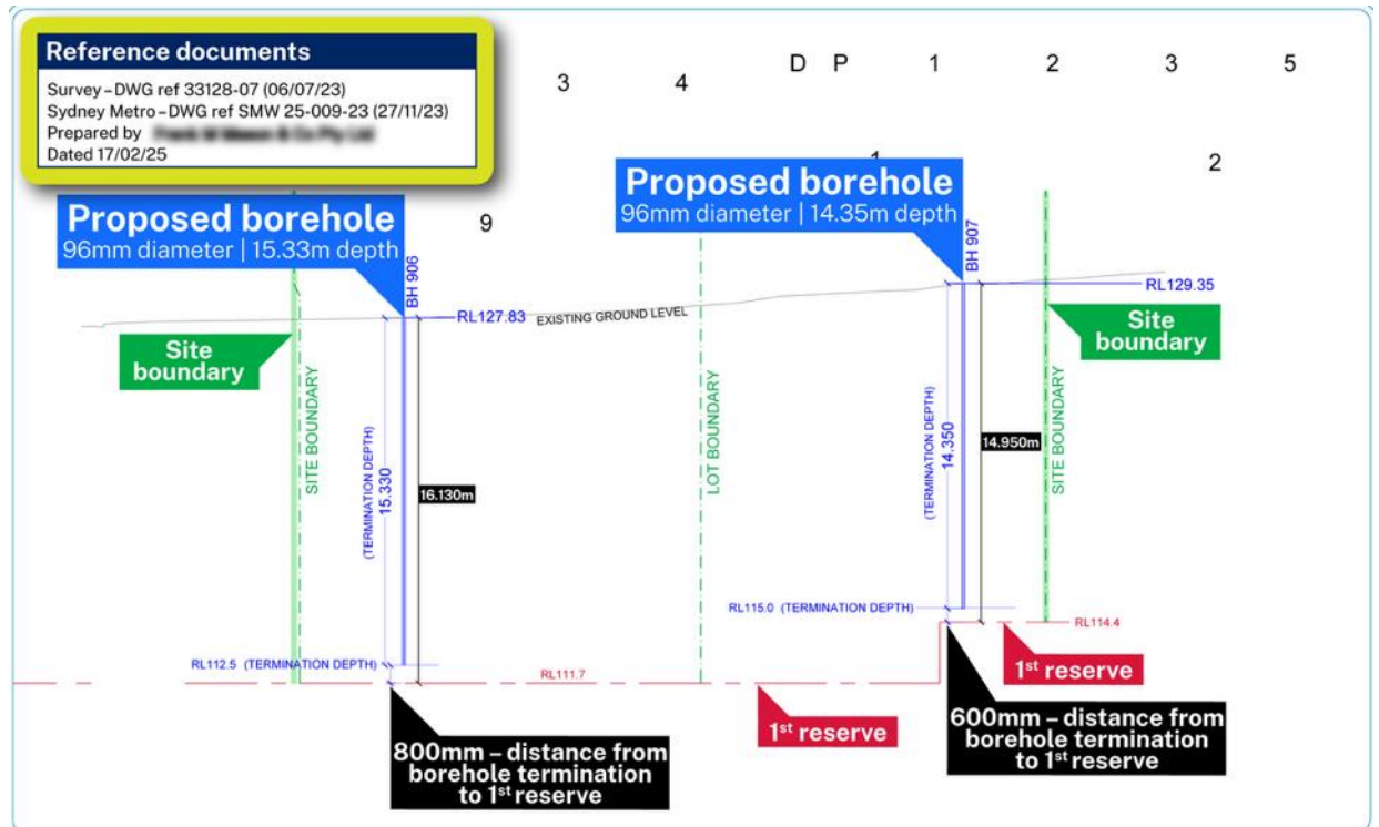
Figure E6 Proposed borehole cross-section
