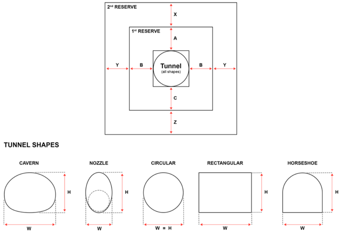
Figure 3.1 Protection reserves for metro tunnels and caverns
