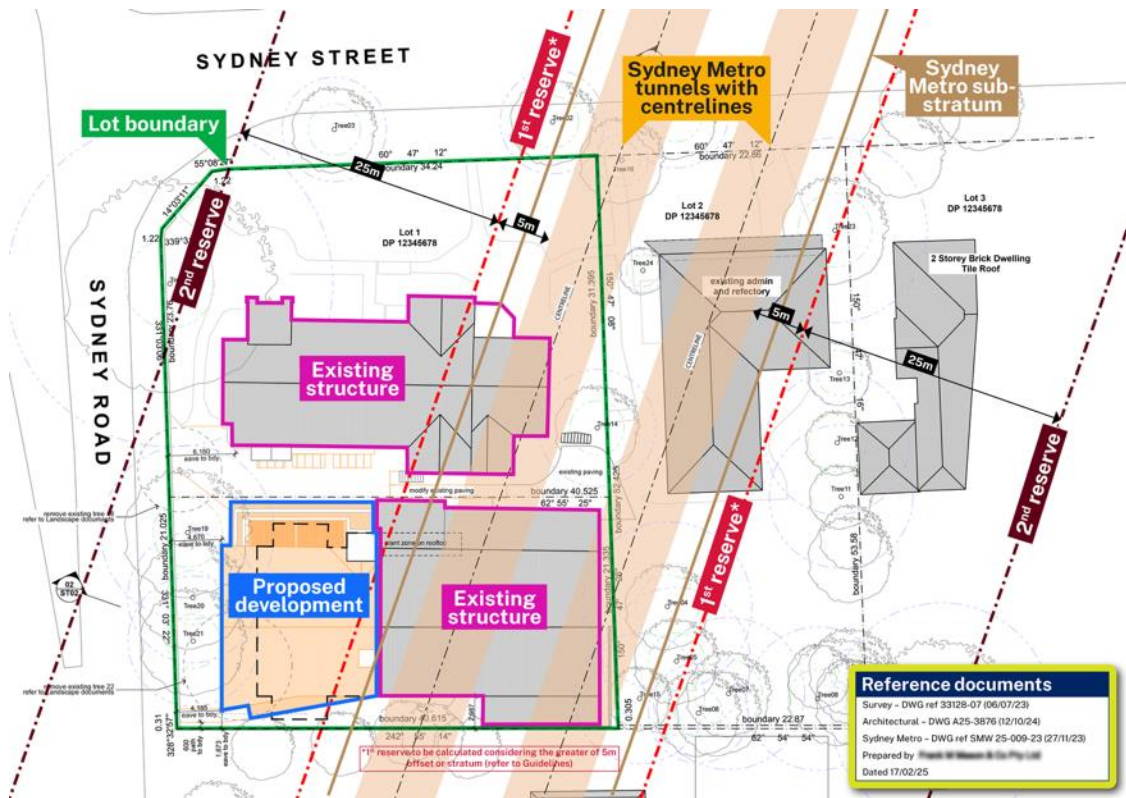
Figure E2 Plan showing Development footprint and relationship to Metro Infrastructure
