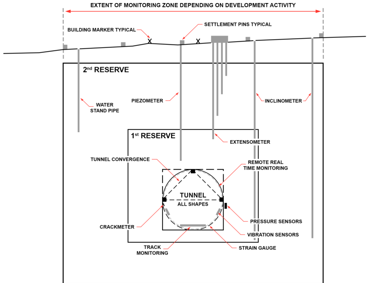
Figure 7.1 Typical monitoring instrument layout
