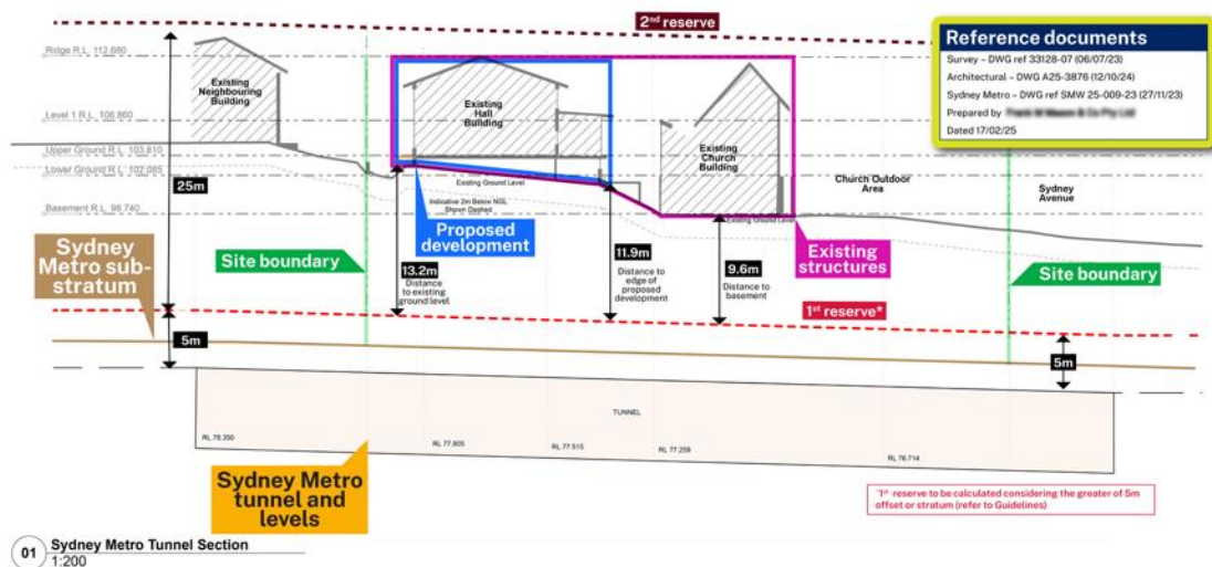
Figure E4 Long section showing Development envelope and relationship to Metro Infrastructure
