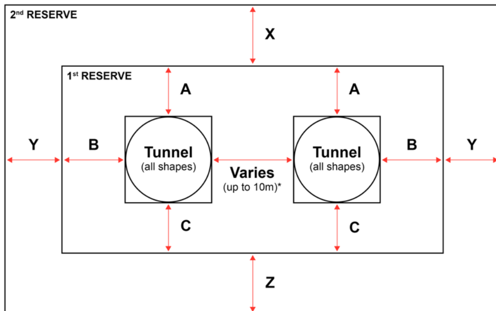
Figure 3.2 Protection reserves for metro parallel running tunnels
