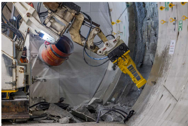
The image above shows excavation being completed within the cross passage.
