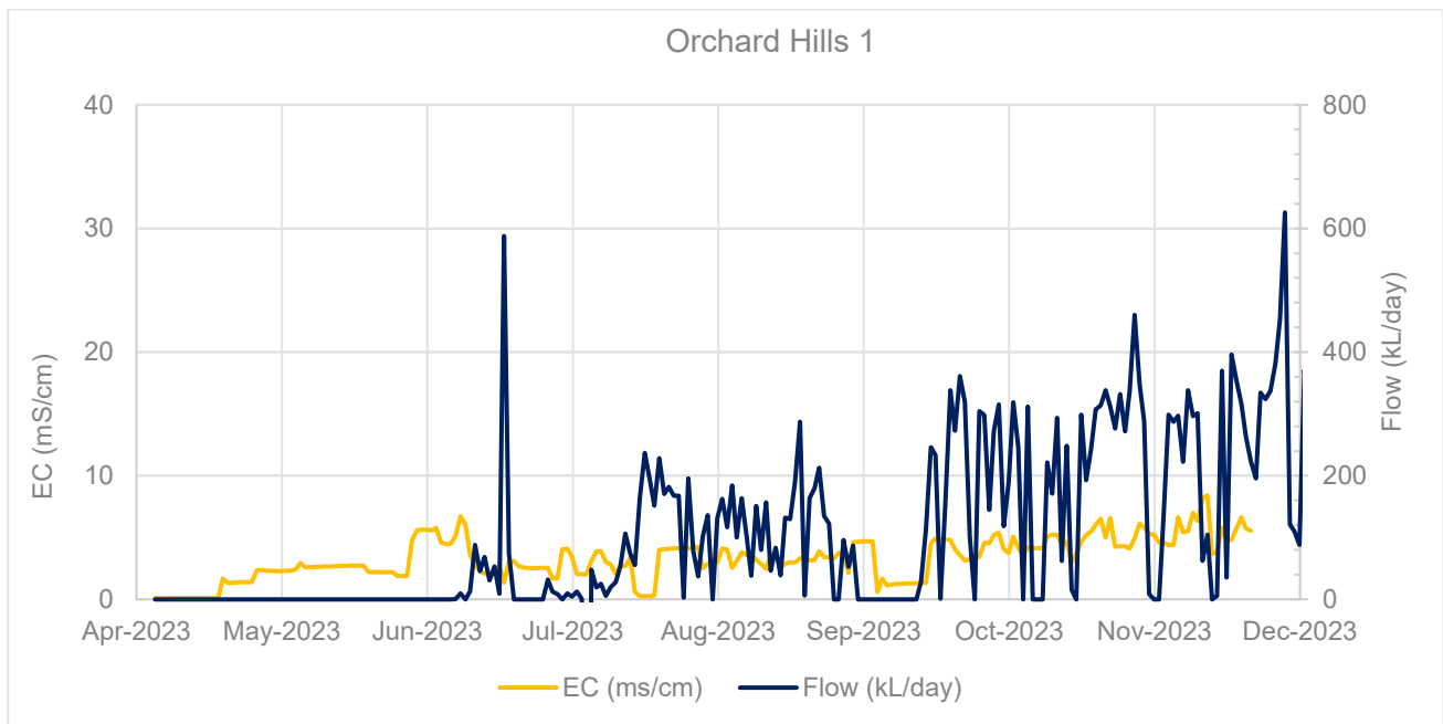
Figure 6-5: Daily inflows and EC at Orchard Hills WTP feed
