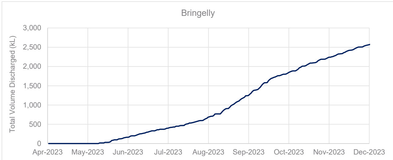
Figure 6-10: Cumulative volume at Bringelly WTP feed
