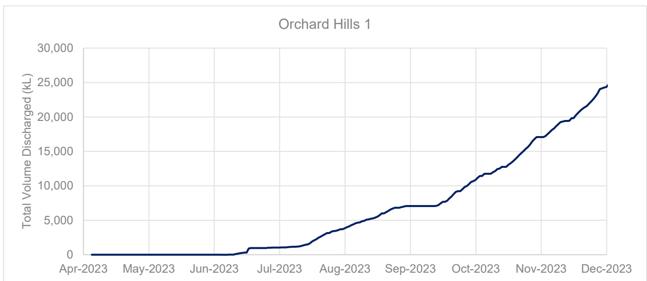
Figure 6-7: Cumulative inflows at Orchard Hills WTP feed
