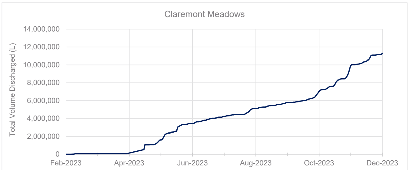
Figure 6-4: Cumulative volumes to Offsite Tanks at Claremont Meadows
