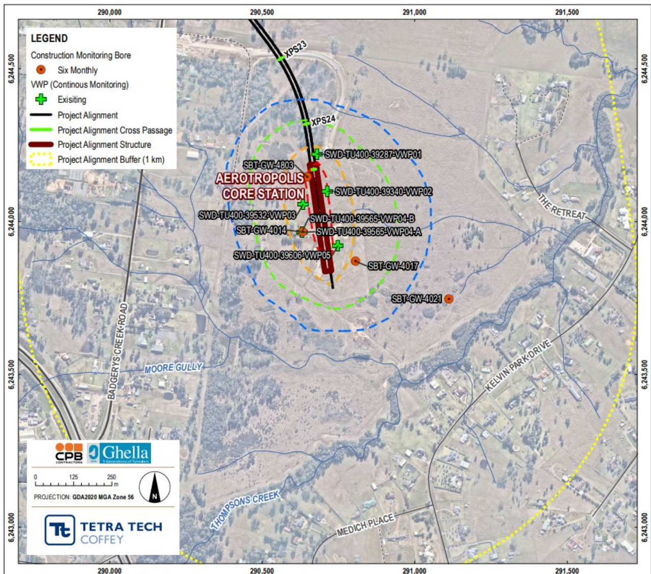
Figure 2-4: Construction groundwater monitoring program – Aerotropolis Core Station
