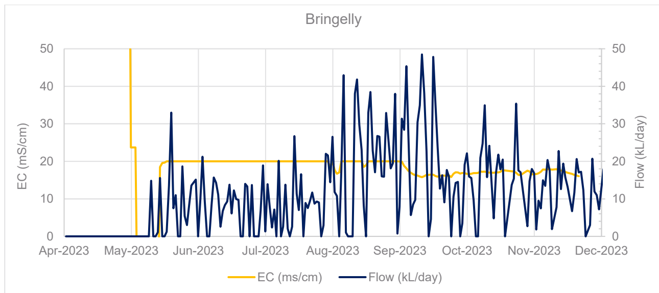
Figure 6-9: Daily inflows and EC at Bringelly WTP feed
