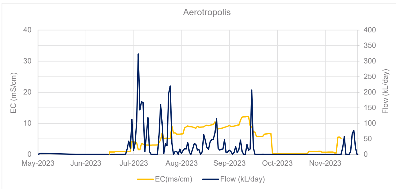
Figure 6-11: Daily inflows and EC at Aerotropolis WTP feed
