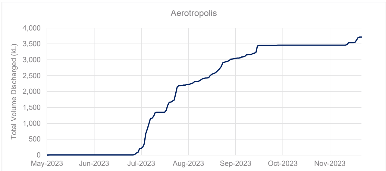
Figure 6-12: Cumulative discharge volume at Aerotropolis
