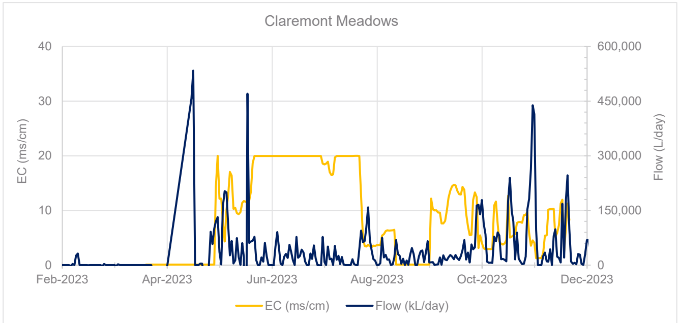
Figure 6-3: Daily inflows and EC at Claremont Meadows Offsite Tanks
