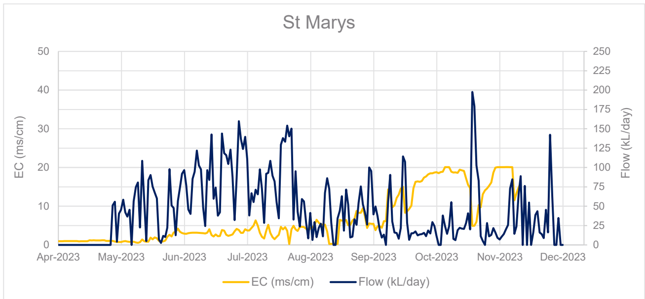
Figure 6-1: Daily inflows and EC at St Marys WTP
