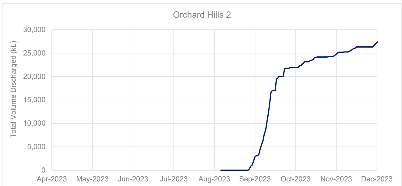
Figure 6-8: Cumulative plant feed volumes to Orchard Hills 2
