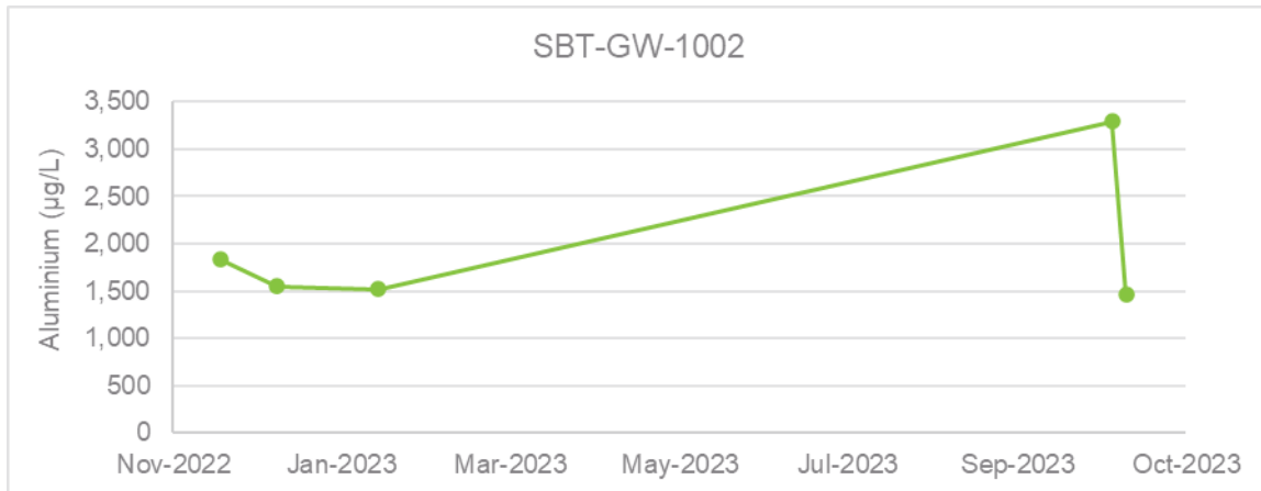
Figure 5-2: Aluminium concentrations in SBT-1002
