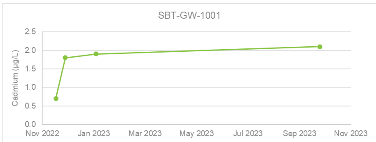
Figure 5-6: Cadmium concentrations in SBT-GW-1001
