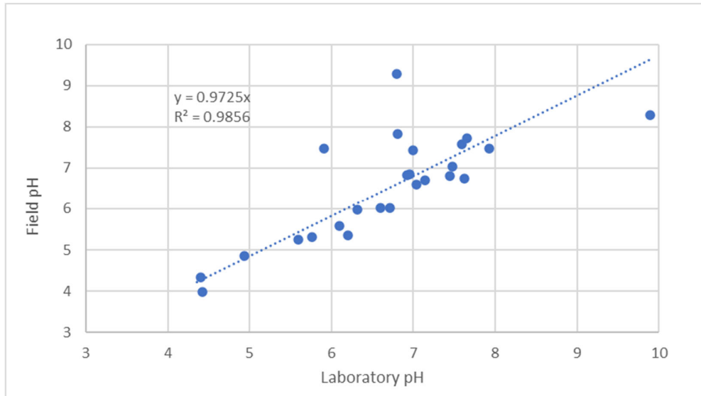
Figure F-1: Laboratory pH versus field pH
