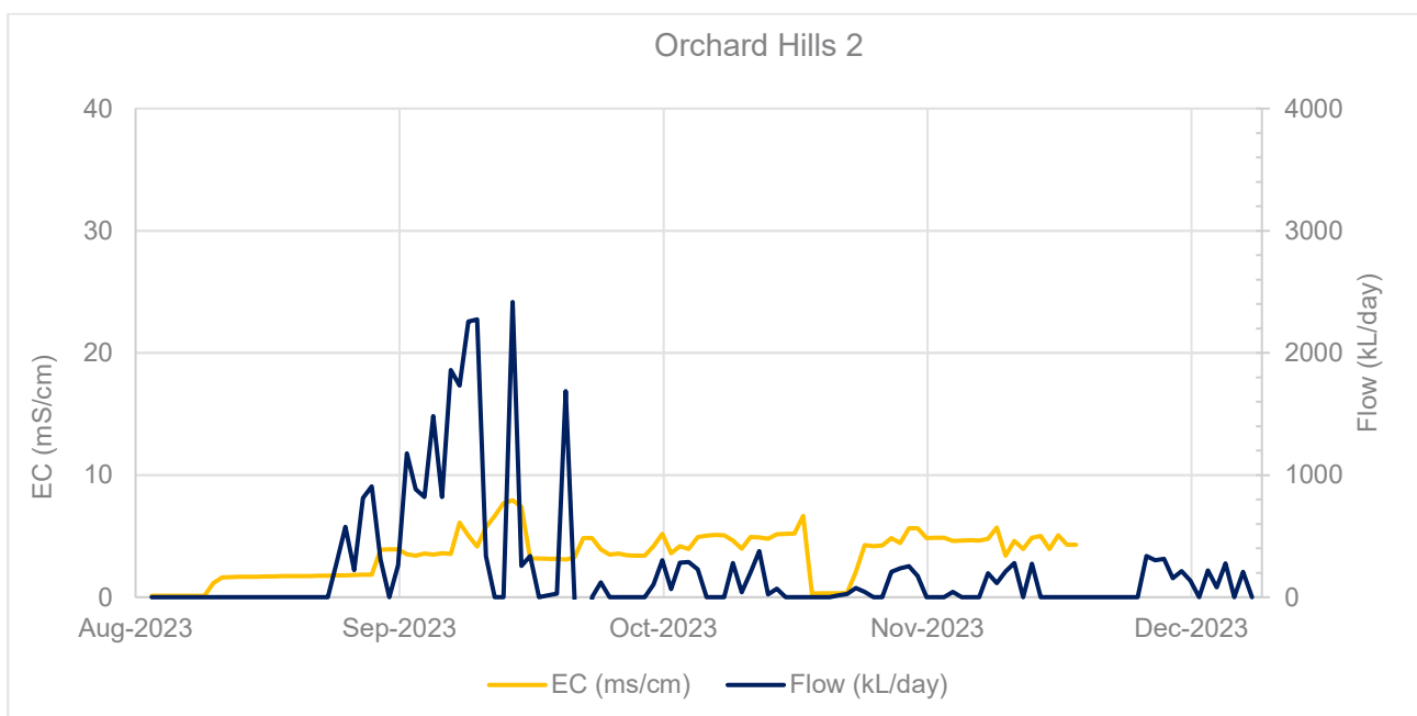
Figure 6-6: Daily plant feed flows and EC at Orchard Hills
