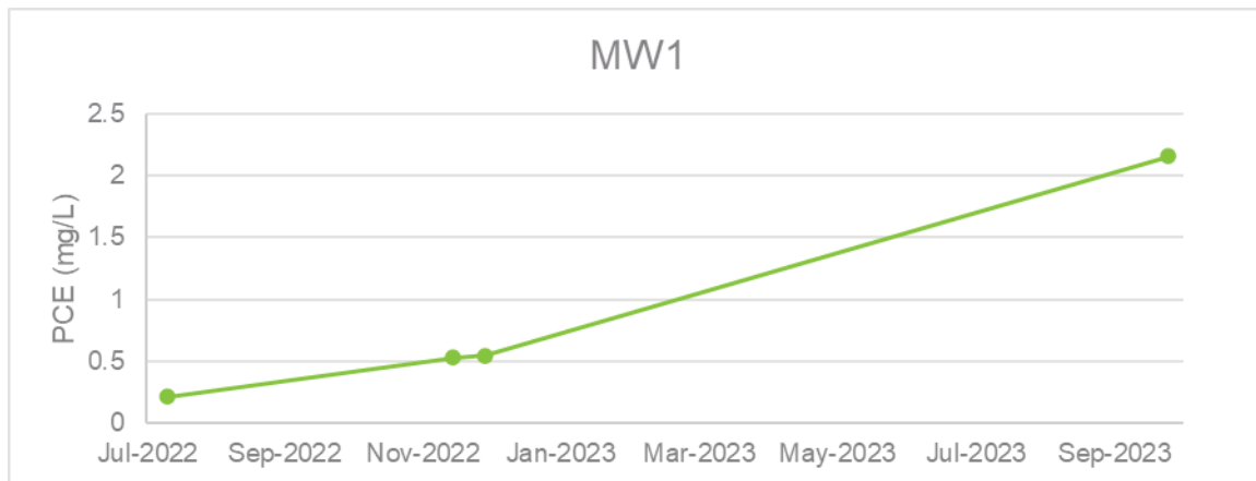
Figure 5-1: PCE concentrations in MW1, St Marys
