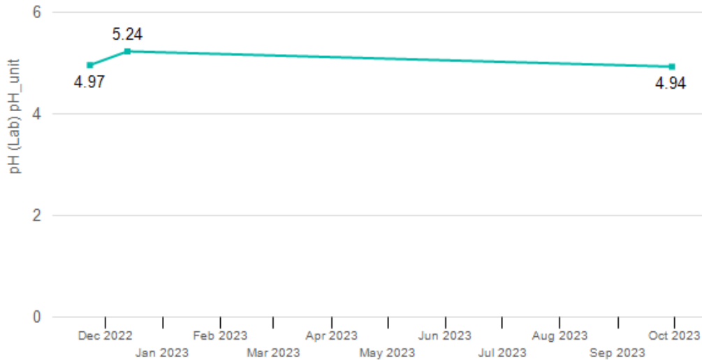
Figure 5-4: Groundwater pH in SBT-GW-1042
