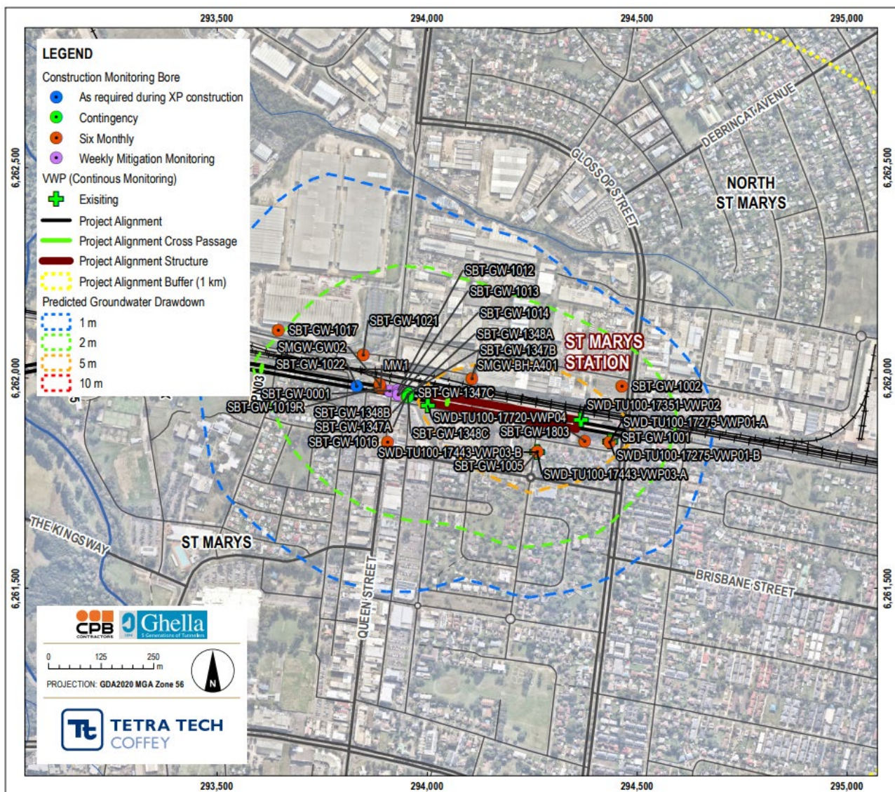
Figure 2-1: Construction groundwater monitoring program – St Marys Station
