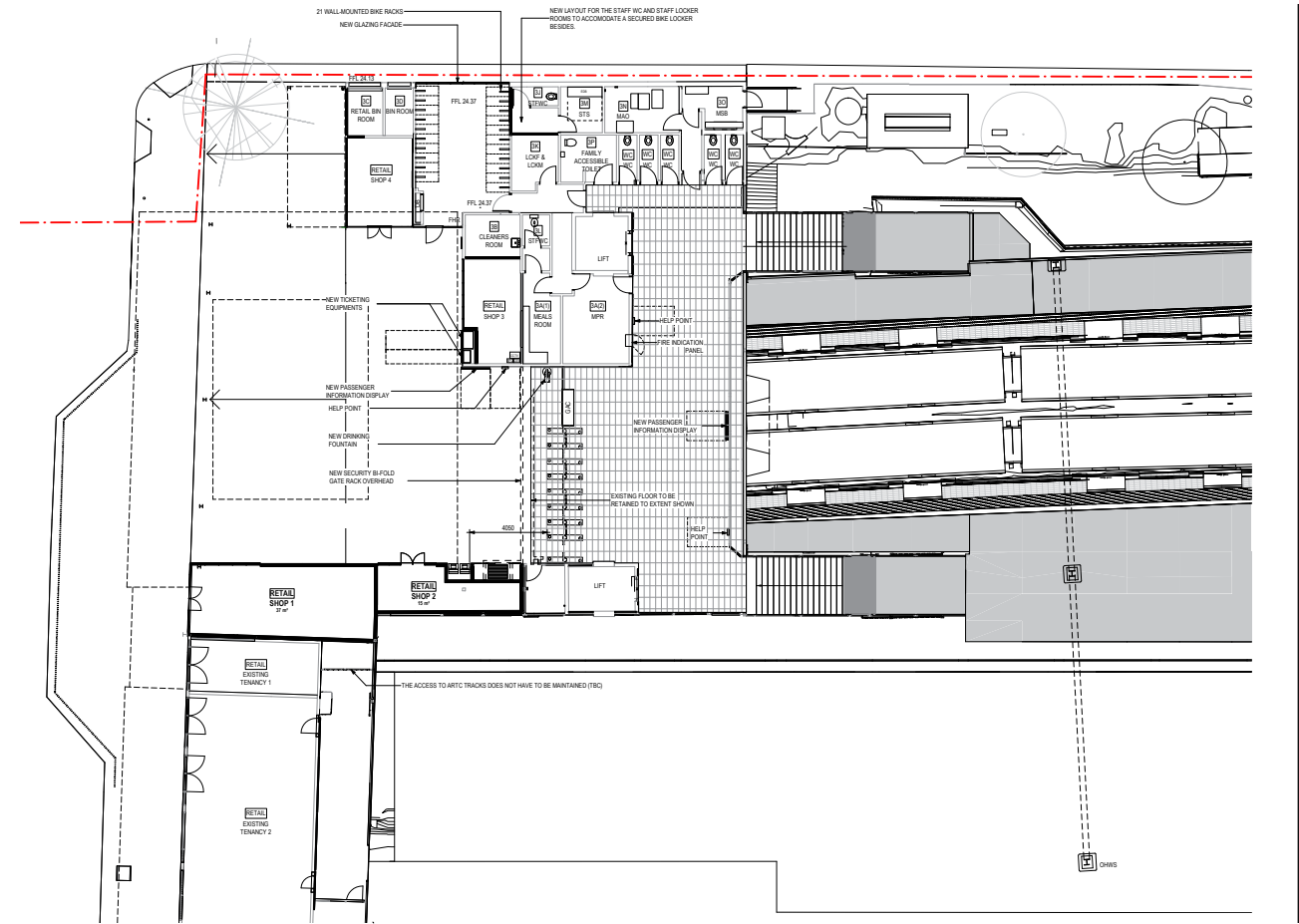
Figure 4.22 Concourse: General arrangement plan
