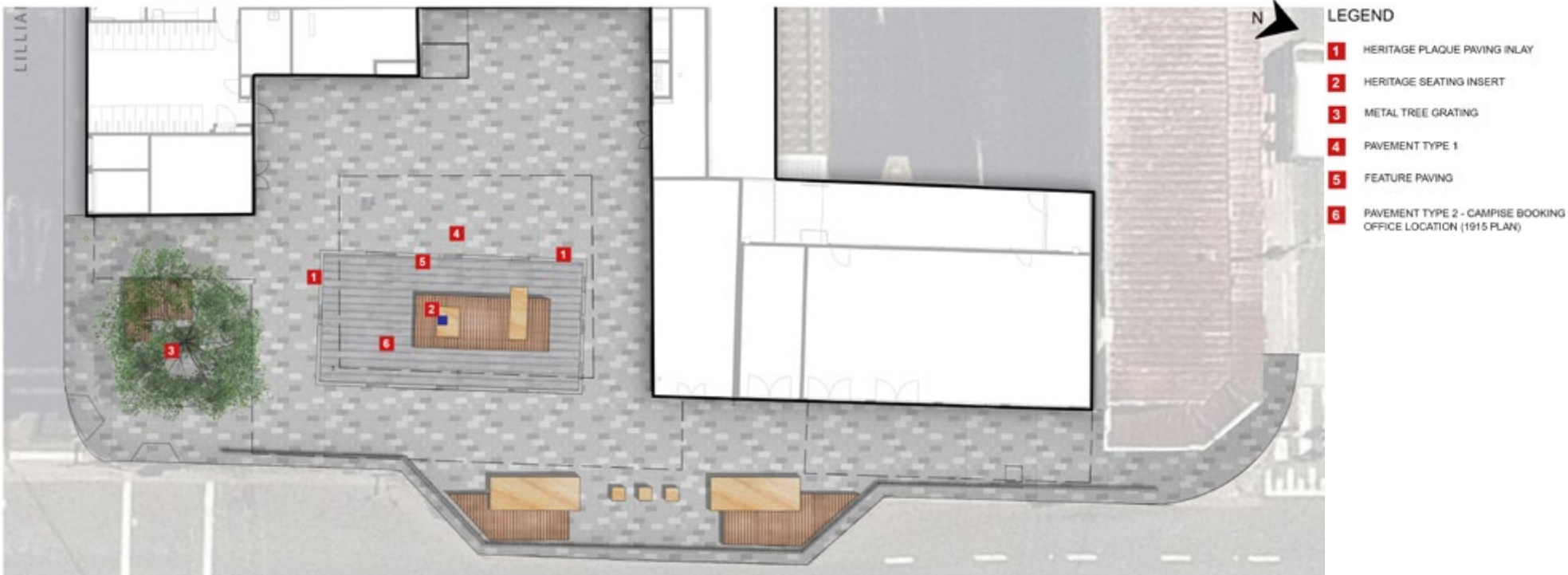
Figure 4.11 Campsie Plaza - Heritage interpretation key plan
