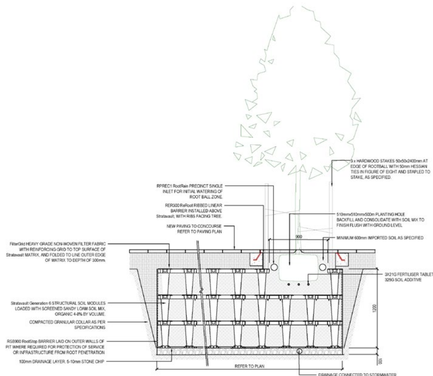
Figure 4.32 Water Sensitive Urban Design soil cell system: detail
