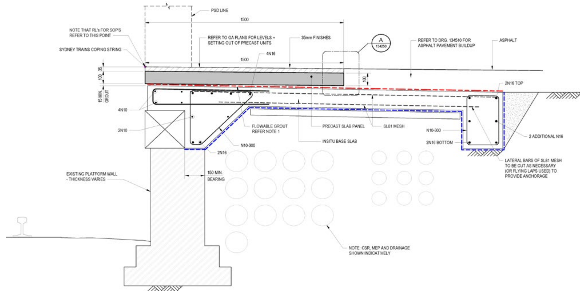
Figure 4.25 Platform edge regrading: detail section
