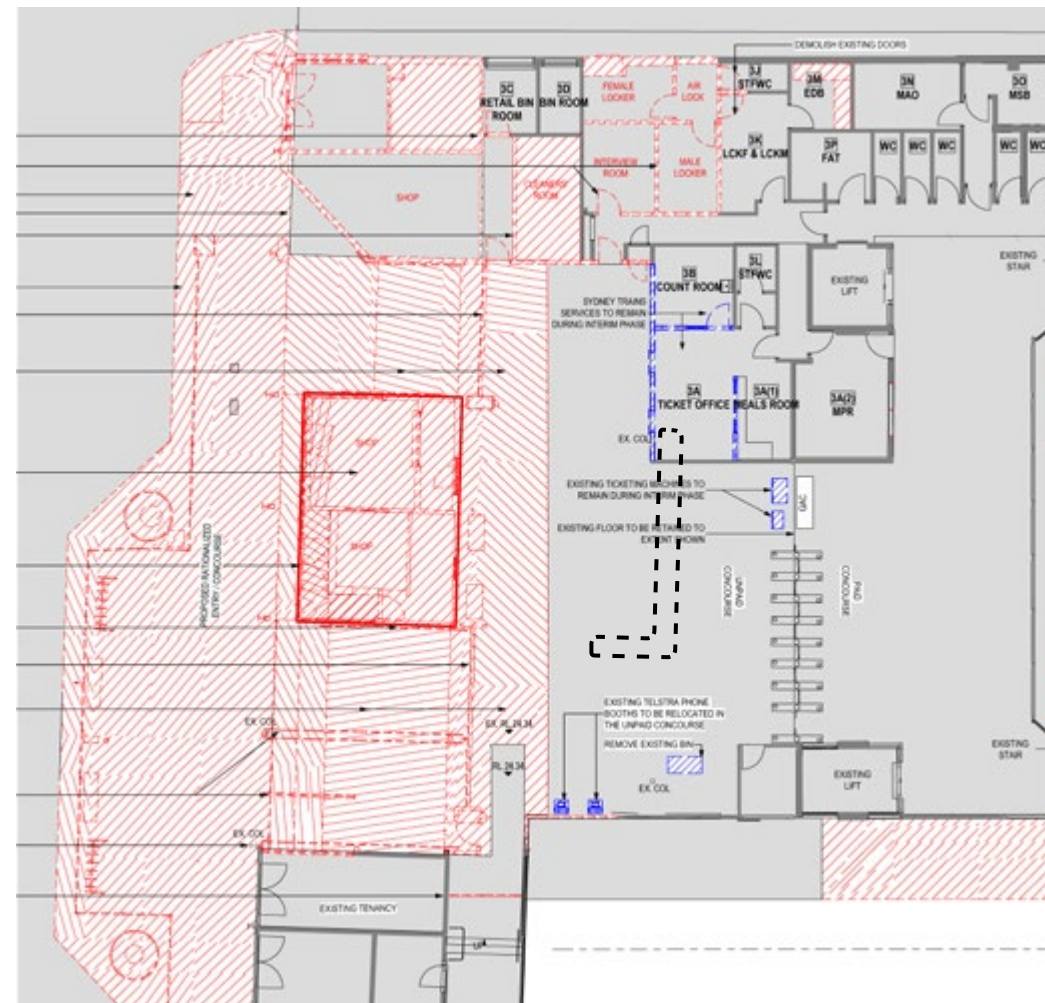
Figure 4.9 Concourse building: Proposed building reconfiguration
