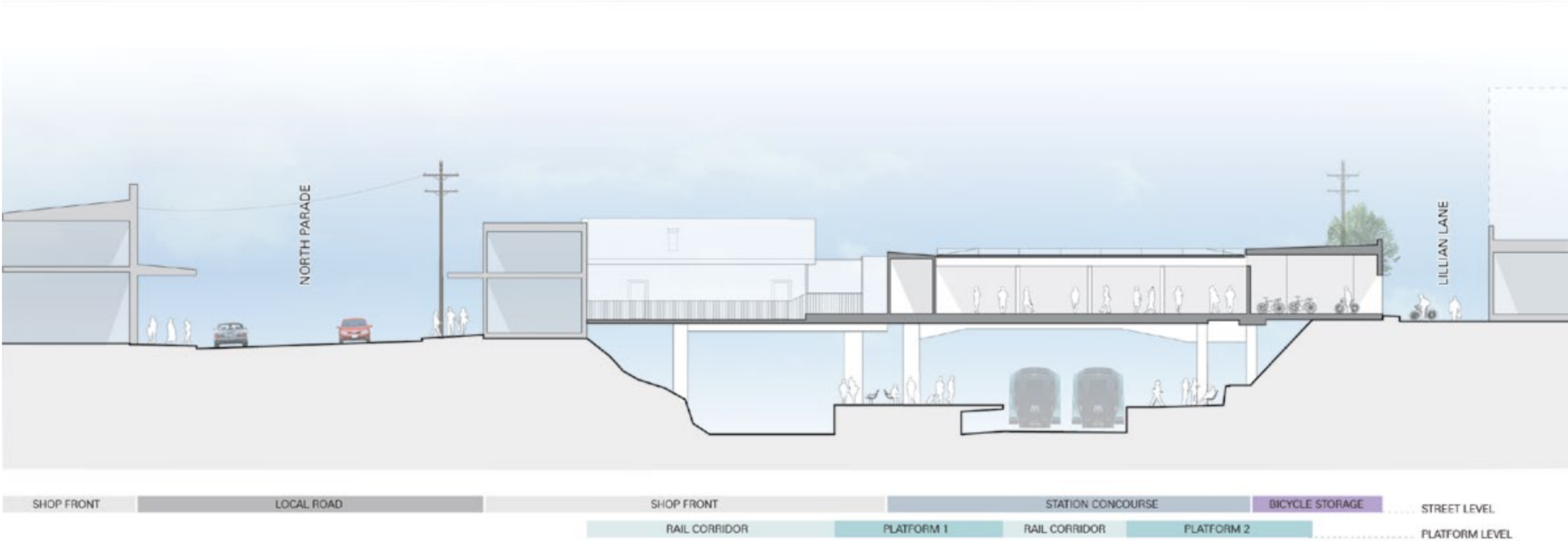
Figure 4.5 Section B Campsie - Short section through concourse and platforms
