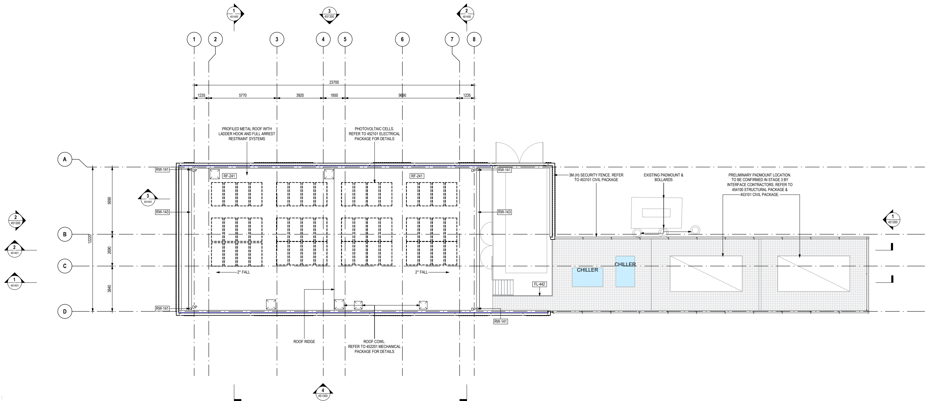
Figure 4.42 Services building plan - Campsie Station
