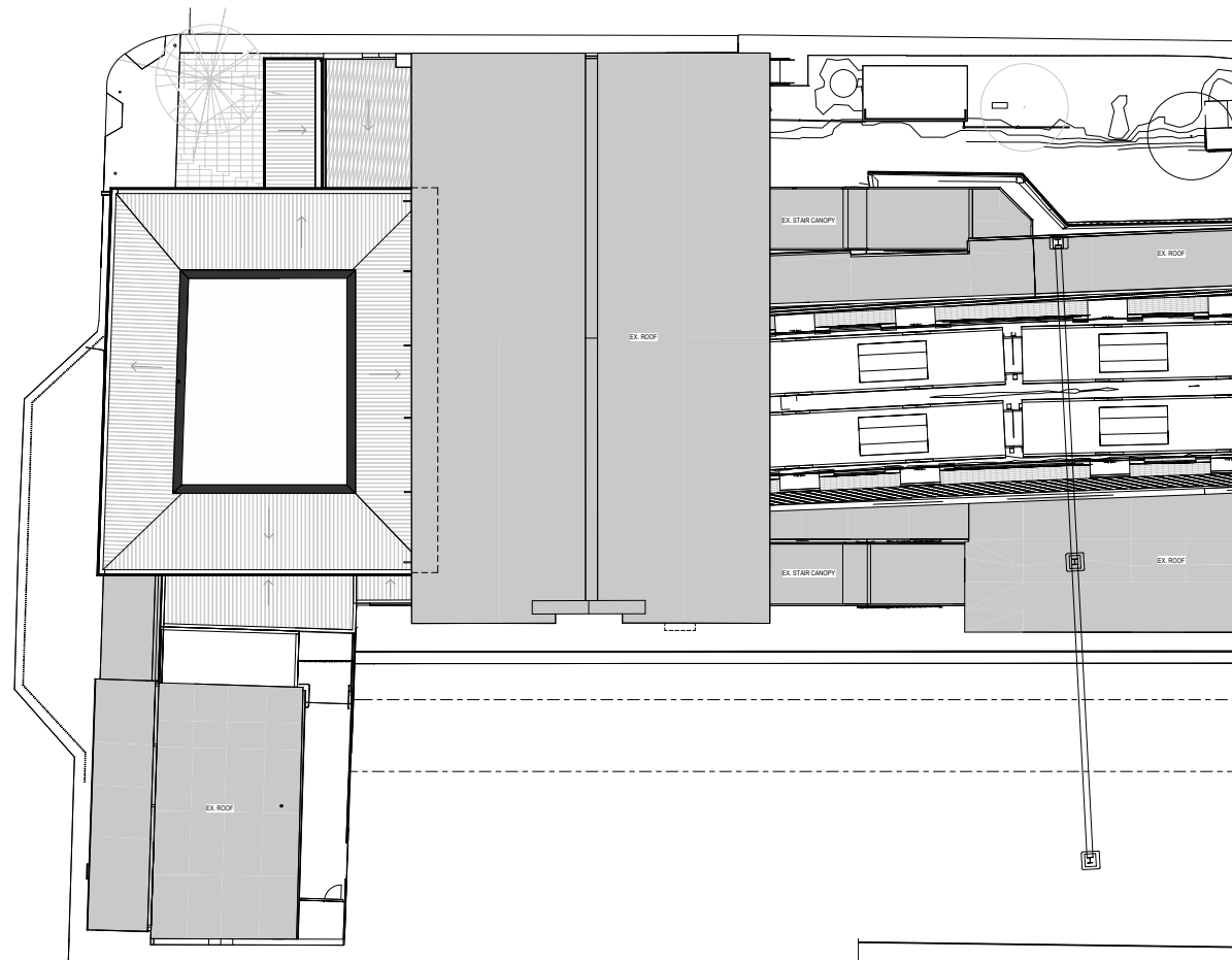
Figure 4.20 Proposed concourse roof
