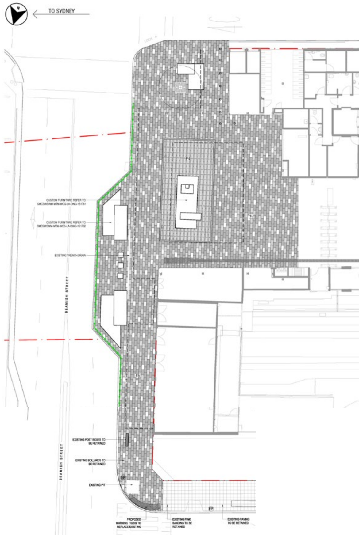
Figure 4.34 Station landscape arrangement
