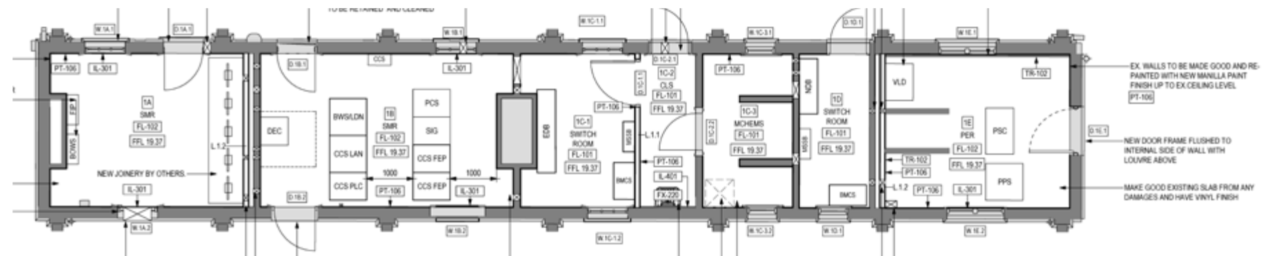
Figure 4.8 Platform Building 1: Detail plan
