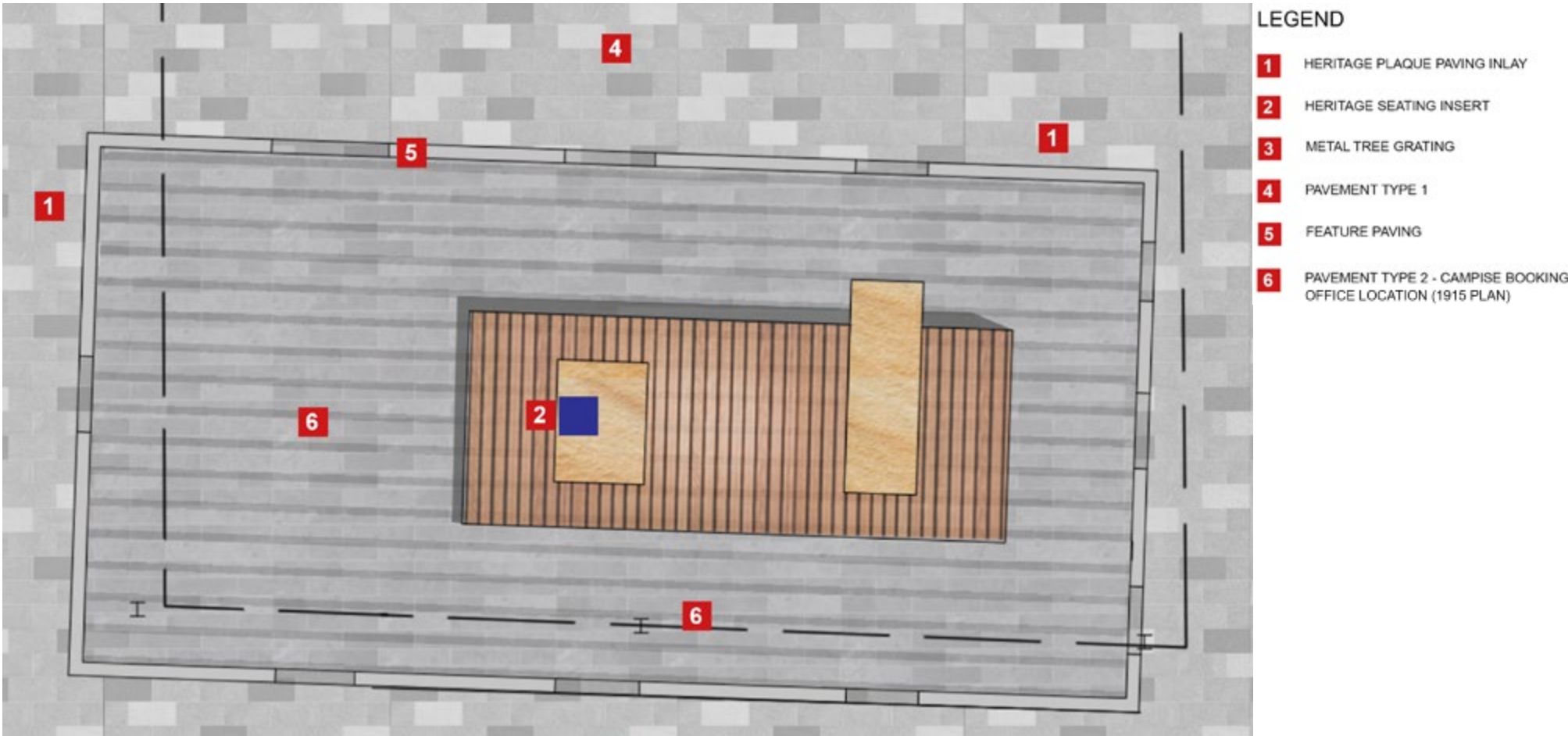
Figure 4.13 Paving inlay and seat element detailed plan
