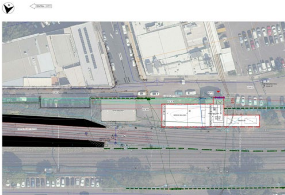
Figure 4.40 Services building site plan - Campsie Station
